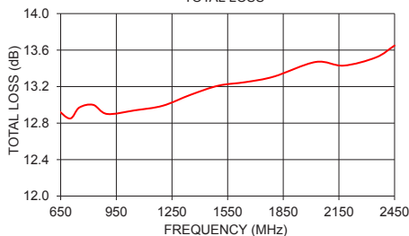
ZC16PD-24+ TOTAL LOSS
