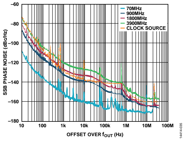
Figure 38. SSB Phase Noise vs. Offset over f_{OUT} , f_{DAC} = 4000 \text{ MSPS} (Two Different DAC Clock Sources Used for Best Composite Curve)
