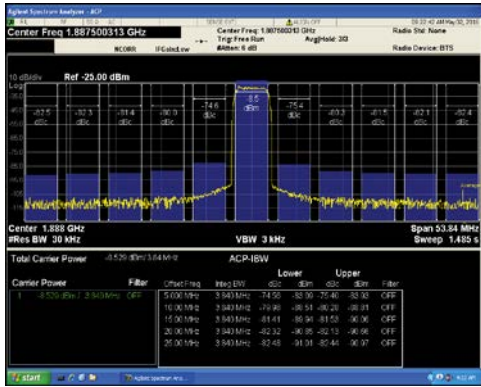
Figure 54. Single-Carrier W-CDMA at 1887.5 MHz
