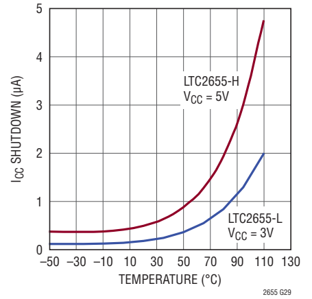
I_{CC} Shutdown vs Temperature
