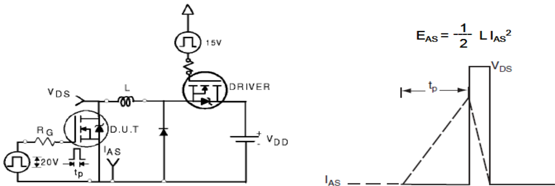
Fig. 17. Unclamped Inductive switching test circuit & waveform
