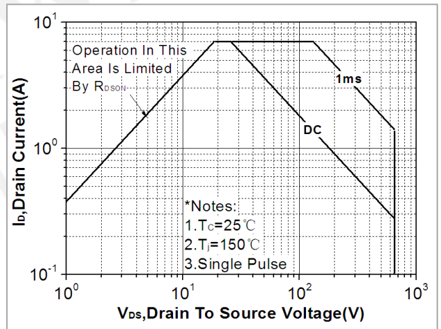
Fig. 10. Maximum safe operating area (TO-251/TO-251N/TO-252)
