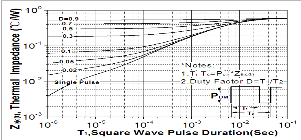
Fig. 13. Transient thermal response curve (TO-251/TO-251N/TO-252)
