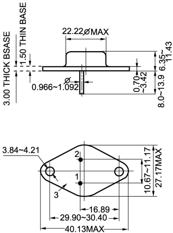
Fig.2 outline dimensions (unindicated tolerance:±0.1mm)
