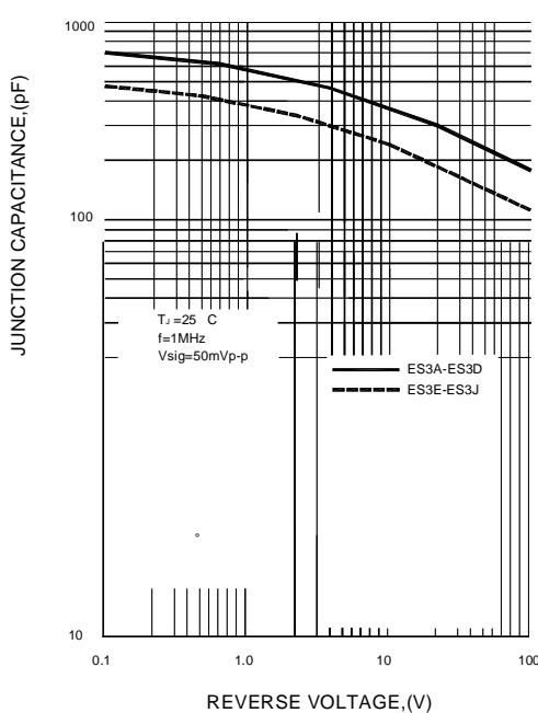
FIG.5-TYPICAL JUNCTION CAPACITANCE
