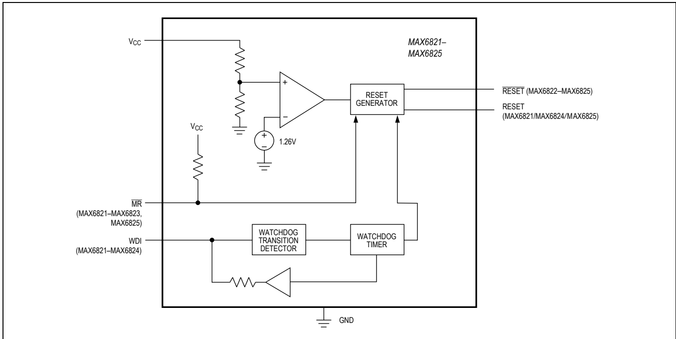
Figure 1. Functional Diagram
