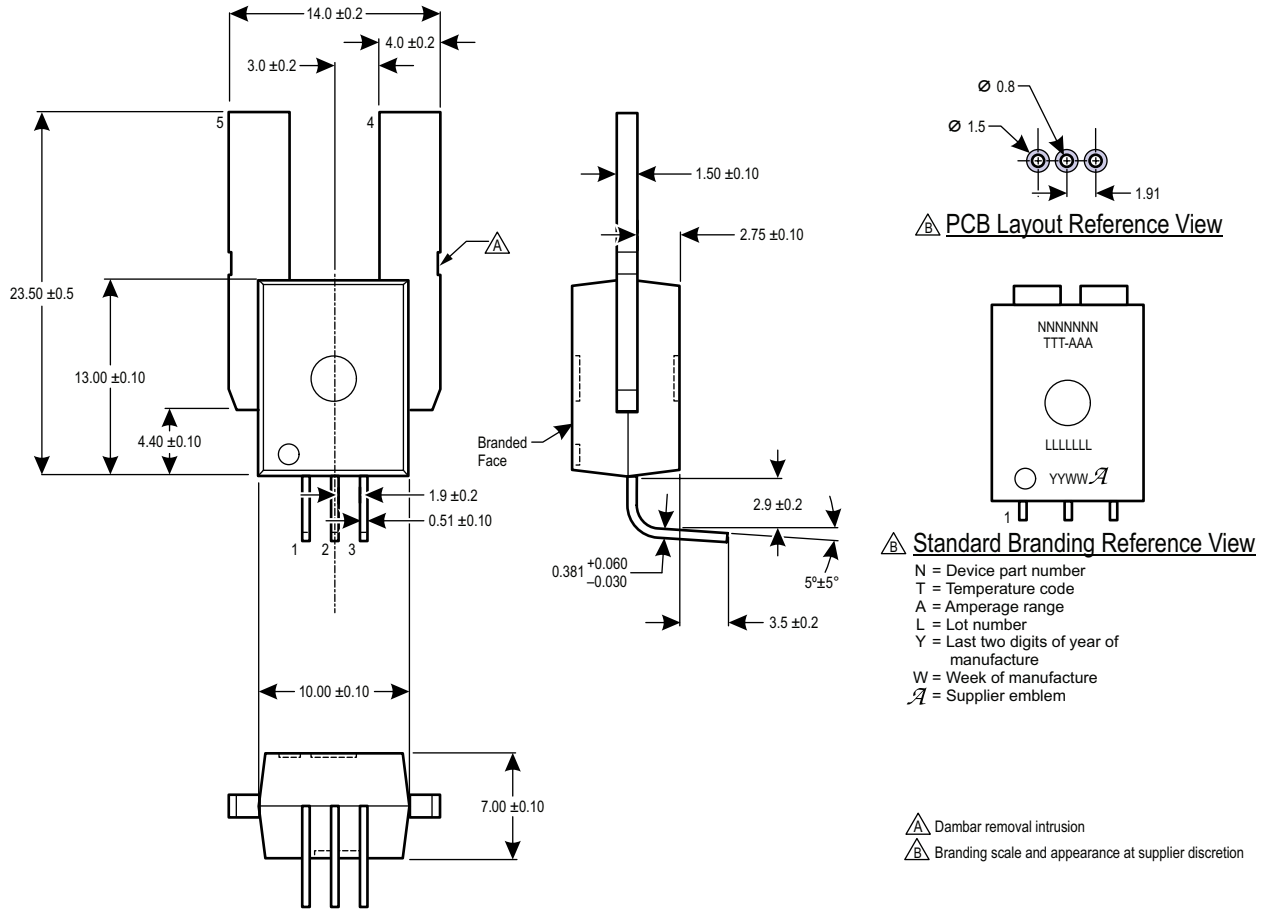
Figure 5: Package CB, 5-Pin, Leadform PSF
