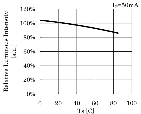
•Solder Temperature vs. Relative Luminous Intensity
