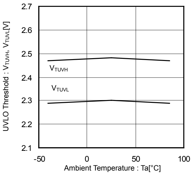
Figure 25. UVLO Threshold Voltage vs Ambient Temperature
