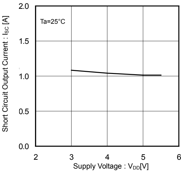
Figure 13. Short Circuit Output Current vs Supply Voltage
