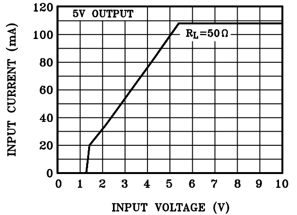
INPUT CURRENT
