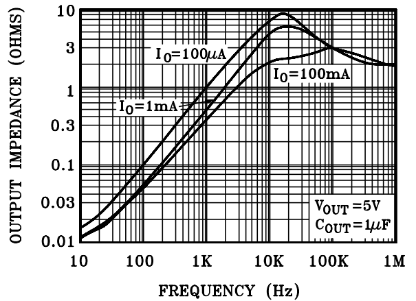
OUTPUT IMPEDANCE
