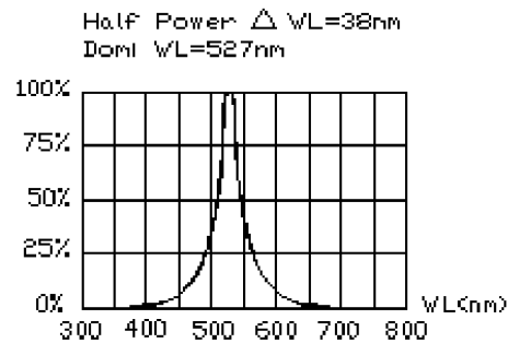
FIG.4 RELATIVE LUMINOUS INTENSITY VS. WAVELENGTH
