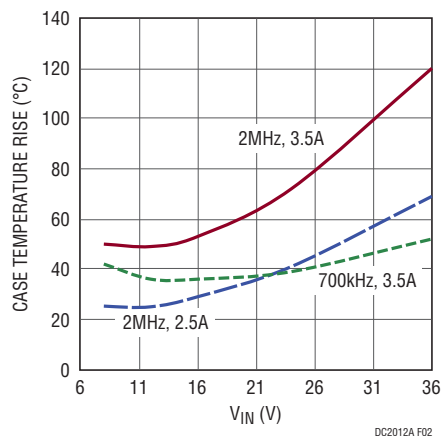
Figure 2. LT8610AB Case Temperature Rise. V_{OUT} = 5V , T_A = 25^\circ C
