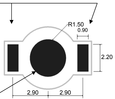
SURFACE MOUNT Recommended Solder Pattern
