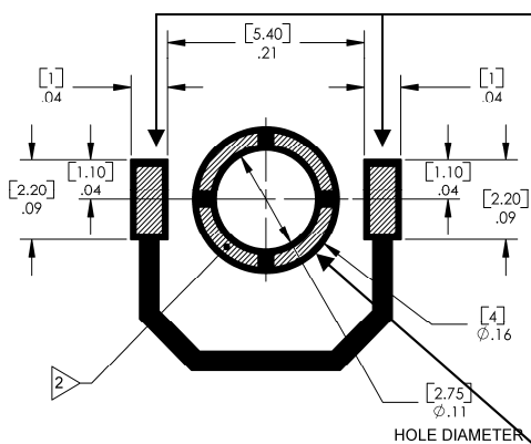
FLUSH MOUNT Recommended Solder Pattern
