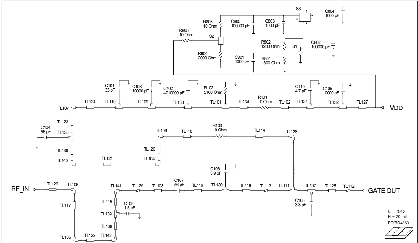
Reference circuit input schematic for f = 960 MHz
