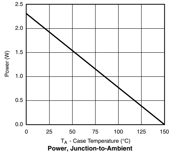
Power, Junction-to-Ambient
