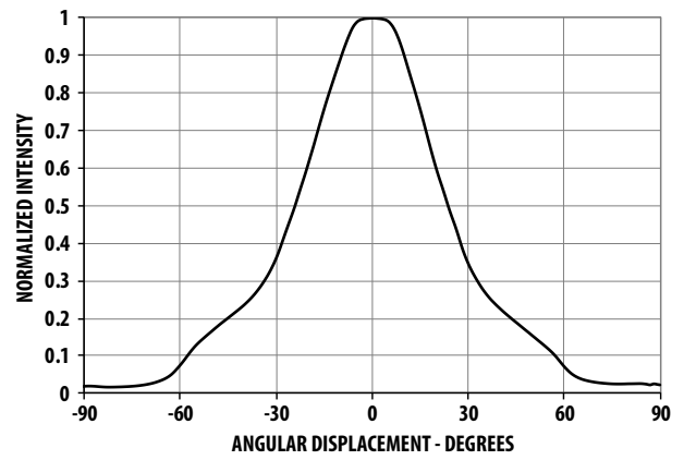
Figure 6b. Radiation Pattern for Minor Axis
