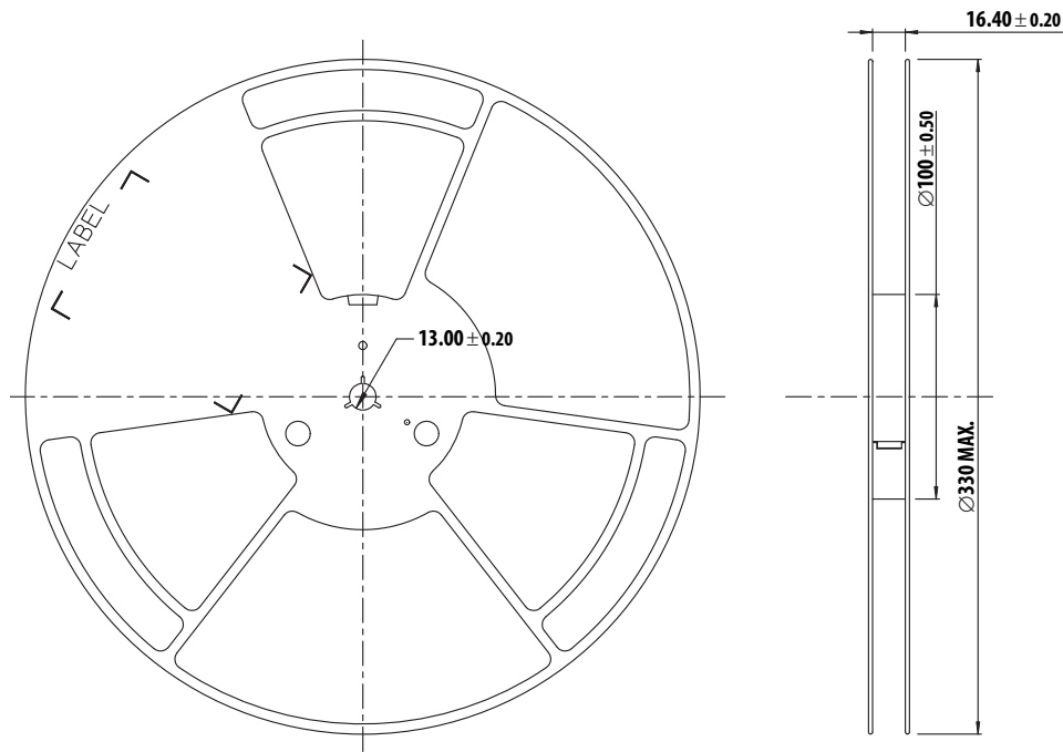
Figure 11. Reel Dimension
