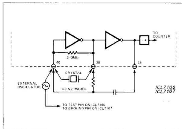
Figure 7. Clock Circuits
