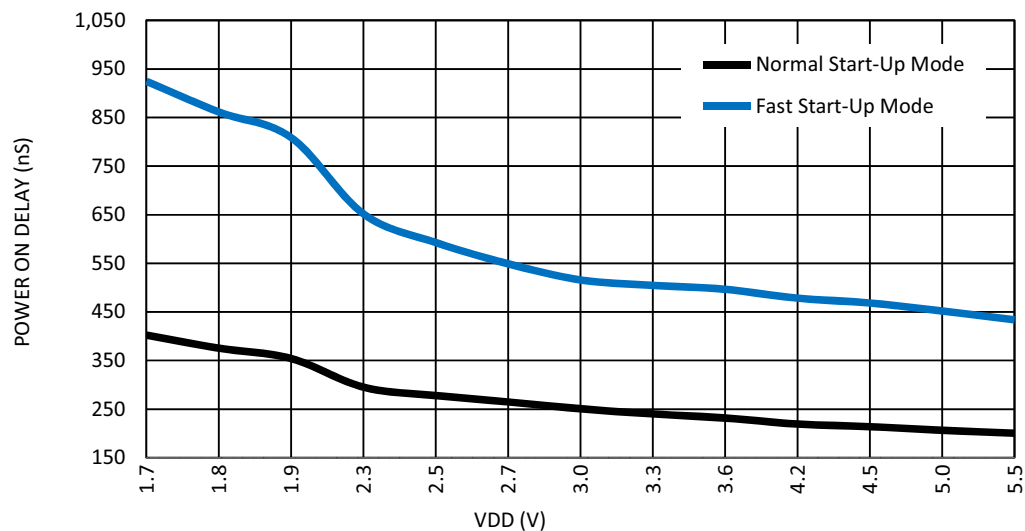
Figure 65. RC Oscillator Maximum Power On Delay vs. VDD at room temperature, OSC0 = 2 MHz
