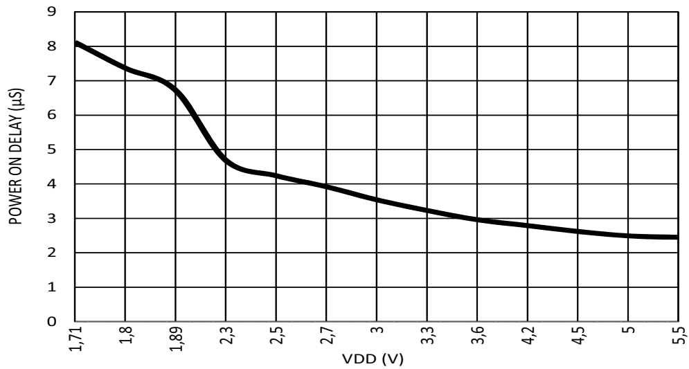
Figure 67. OSC1 (25 MHz) Maximum Power On Delay vs. VDD at room temperature
