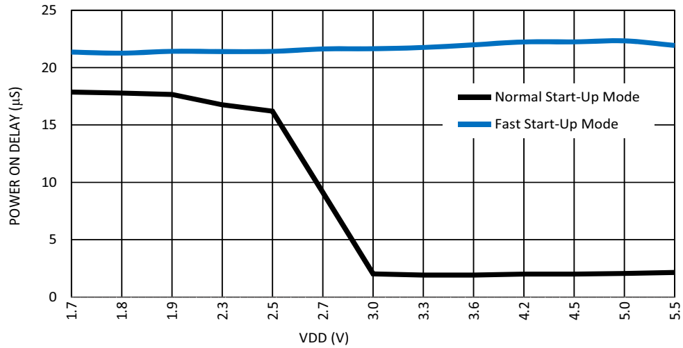
Figure 66. RC Oscillator Maximum Power On Delay vs. VDD at room temperature, OSC0 = 25 kHz
