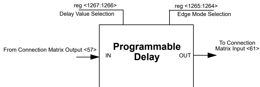
Figure 58. Programmable Delay
