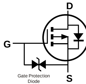
Internal Schematic
