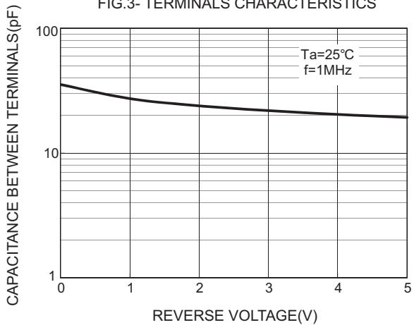
FIG.3- TERMINALS CHARACTERISTICS
