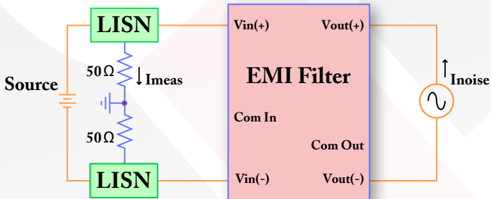
Figure B: Differential-Mode Current Attenuation, I_{meas} / I_{noise}
