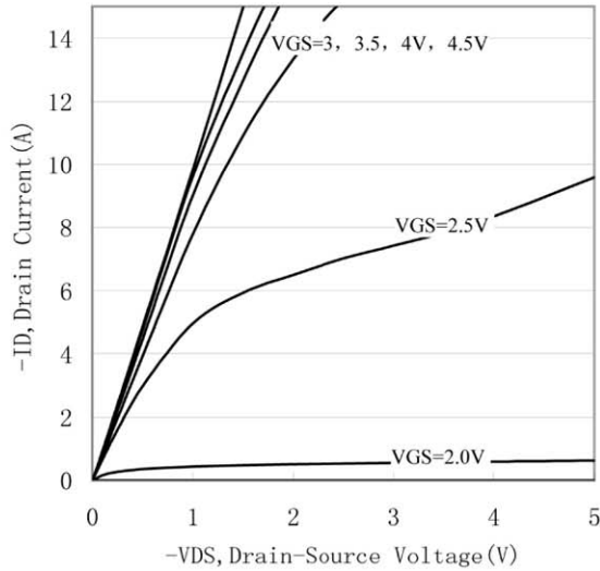
Figure 1. Output Characteristics
