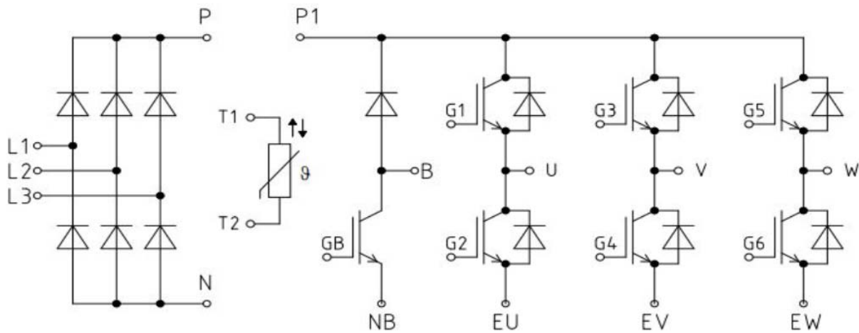
Figure11. Circuit Diagram
