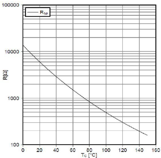
Figure11. NTC-Thermistor-temperature characteristic
