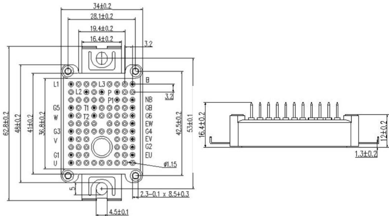
Figure12. Package Dimensions (mm)
