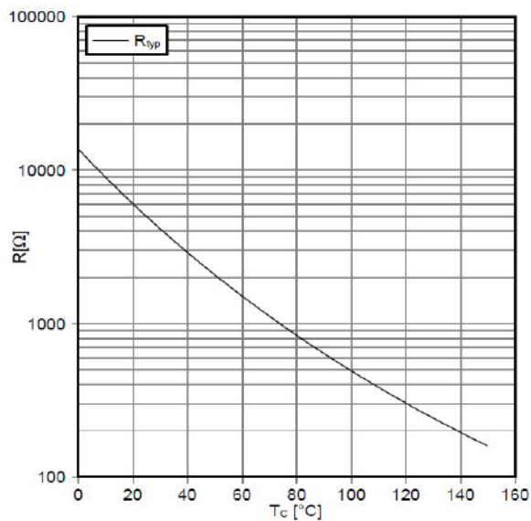
Figure11. NTC-Thermistor-temperature characteristic
