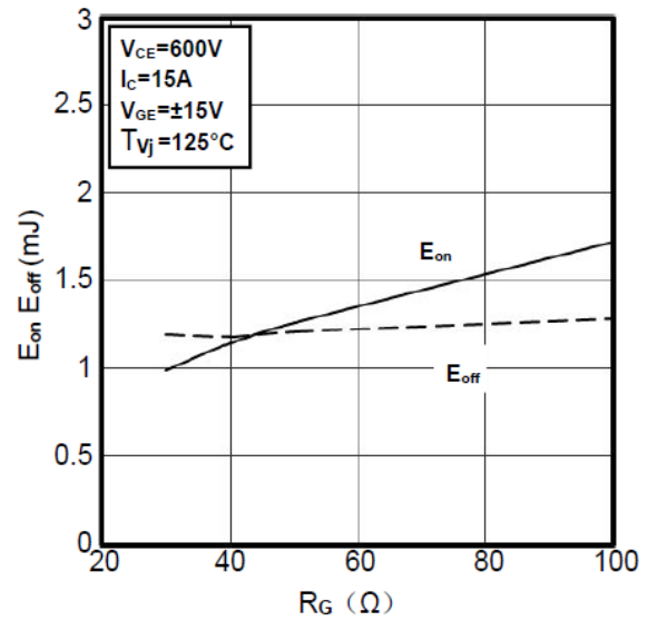
Figure4. Switching Energy vs. Gate Resistor
