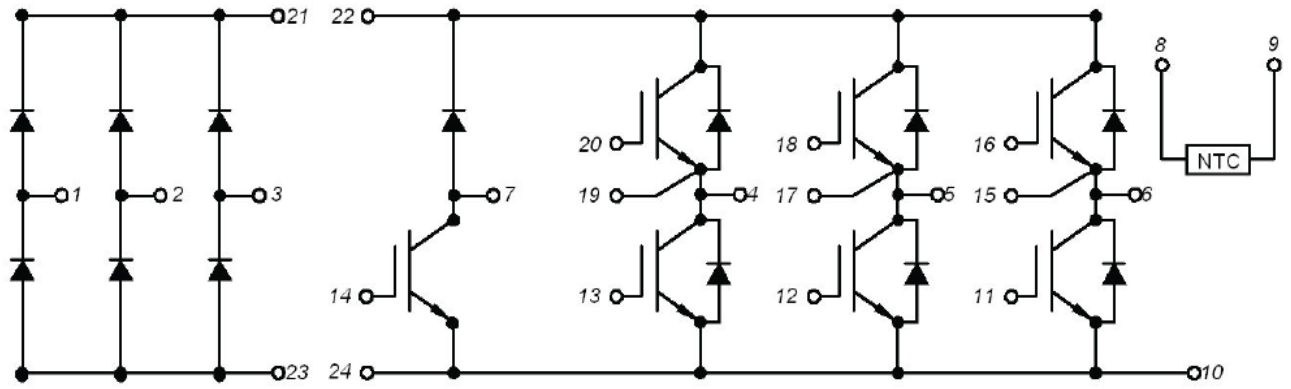
Figure11. Circuit Diagram
