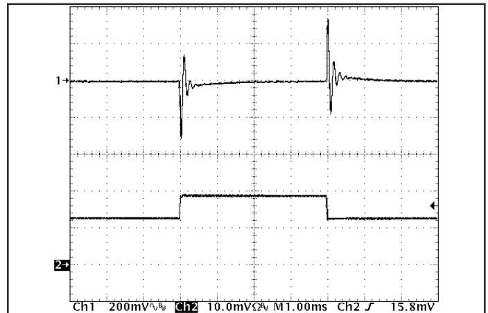
Figure 10: Output voltage response to step-change in load current (50%-75%-50% of Iout(max); dl/dt = 5A/\mu s ). Load cap: 470µF, 15mΩ ESR tantalum cap and 1µF ceramic cap. Top trace: Vout (200mV/div), Bottom Trace: Iout (20A/div).
