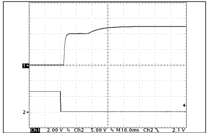
Figure 8: Turn-on transient at zero load (10 ms/div). Top Trace: Vout (2V/div). Bottom Trace: ON/OFF input (5V/div)
