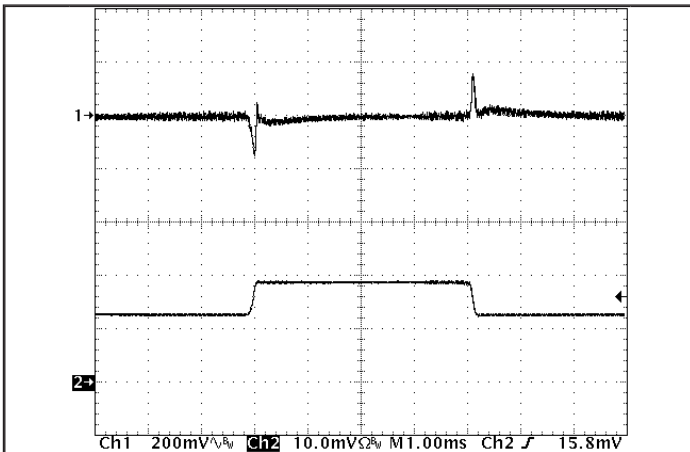
Figure 9: Output voltage response to step-change in load current (50%-75%-50% of Iout(max); dl/dt = 0.1A/\mu s ). Load cap: 15µF, 450mΩ ESR tantalum cap and 1µF ceramic cap. Top trace: Vout (200mV/div), Bottom Trace: Iout (20A/div).
