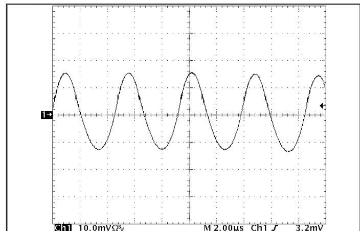
Figure 12: Input Terminal Ripple Current, i_c , at full rated output current and nominal input voltage with 10µH source impedance and 47µF electrolytic capacitor (200mA/div). (See Figure 11).
