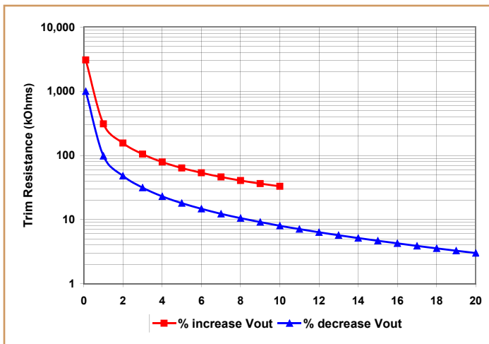
Figure C: Trim Graph
