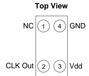
Figure 1. Pin Assignment
