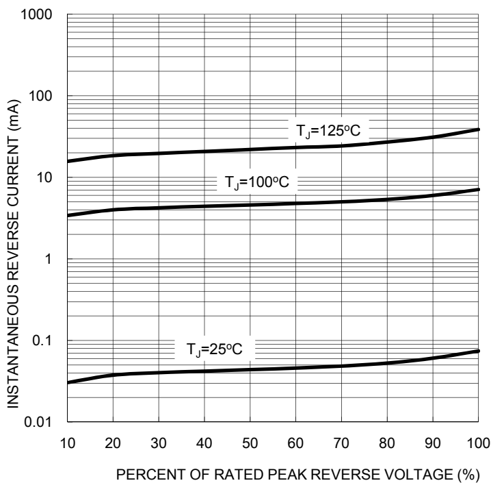
FIG. 3 TYPICAL REVERSE CHARACTERISTICS PER LEG
