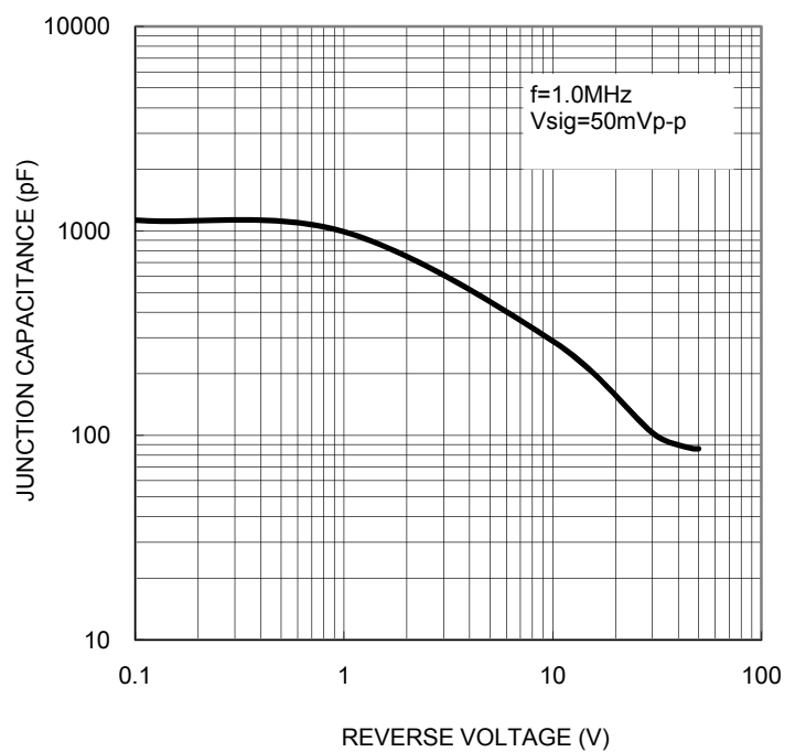
FIG. 4 TYPICAL JUNCTION CAPACITANCE PER LEG
