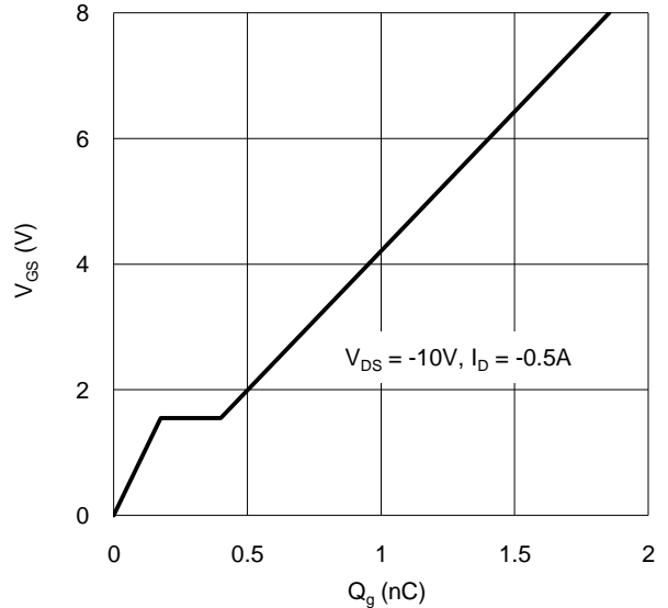
Figure 10. Gate Charge
