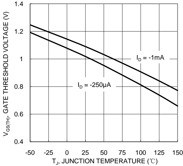
Figure 7. Gate Thershold Variation vs. Junction Temperature
