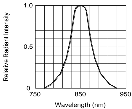
FIG.1 SPECTRAL DISTRIBUTION
