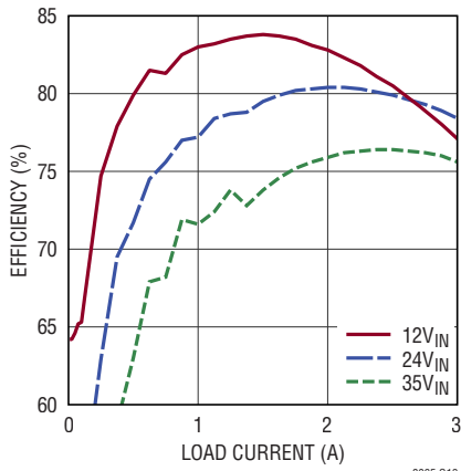
Efficiency, V_{OUT} = -3.3\text{V} , BIAS tied to LTM8065 GND
