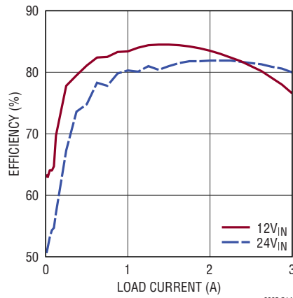
Efficiency, V_{OUT} = -5\text{V} , BIAS tied to LTM8065 GND
