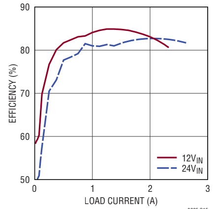
Efficiency, V_{OUT} = -8\text{V} , BIAS tied to LTM8065 GND
