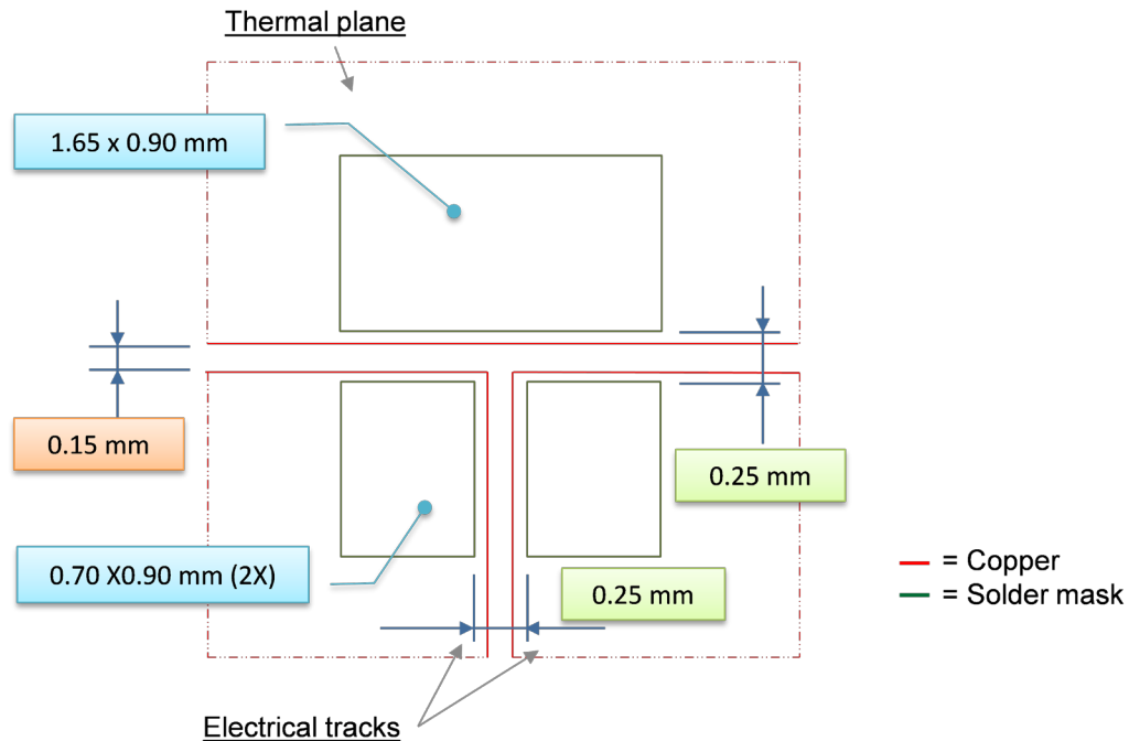
Figure 7. Recommended standard layout.
