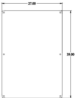
INNER PANEL
