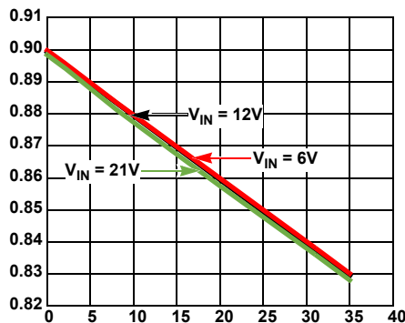
Figure 2. V_{GT}/VR B Load Line = 2m\Omega
