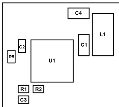
Component Placement
