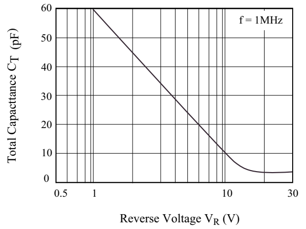
C_R - V_R
