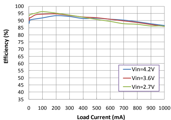
Efficiency VS Load Current, Vout=2.5V
