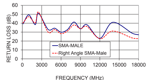
086-11SMRSM+ RETURN LOSS
