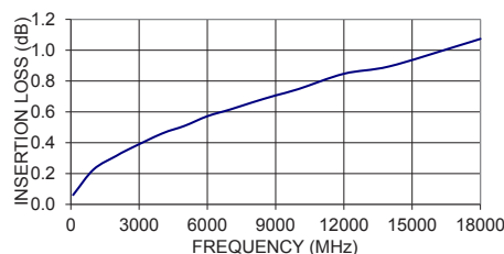
086-11SMRSM+ INSERTION LOSS
