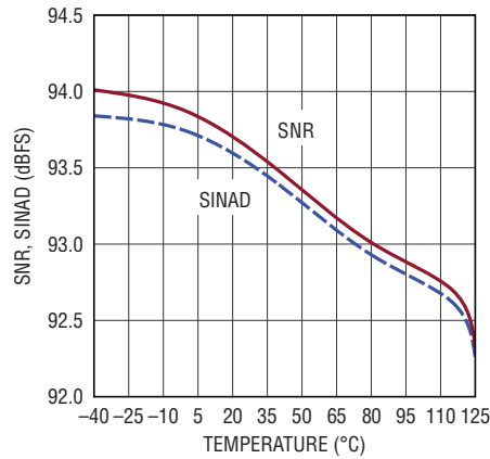
SNR, SINAD vs Temperature, f_{IN} = 1\text{kHz}
