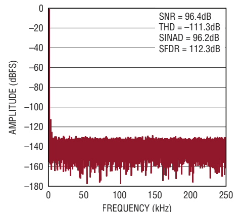
32k Point FFT f_{SAMPL} = 500\text{kps} , f_{IN} = 1\text{kHz} , \text{REF}_{BUF} = 5\text{V}
