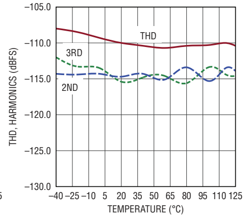
THD, Harmonics vs Temperature, f_{IN} = 1\text{kHz}
