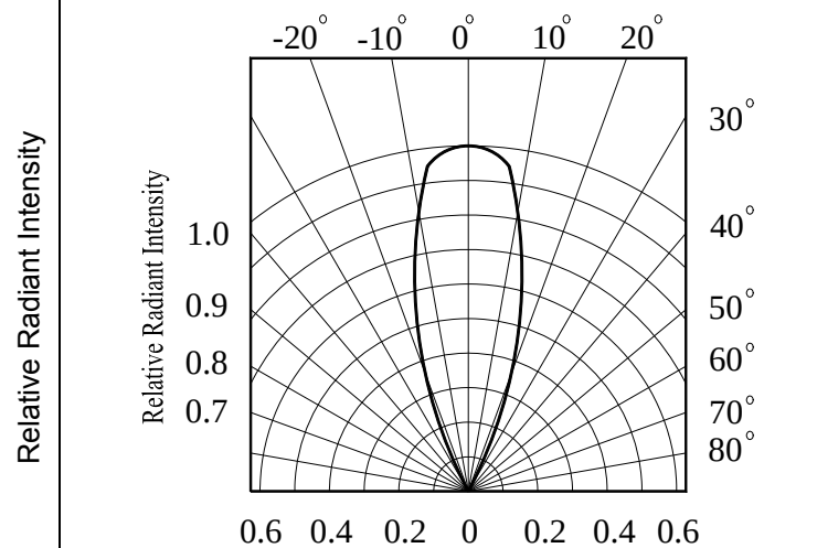
Fig.4 Relative Radiant Intensity vs. Angular Displacement
