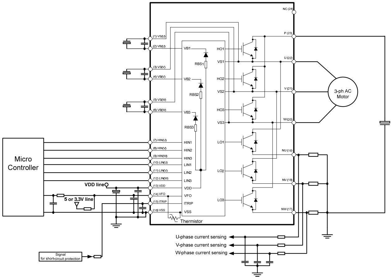
Figure 9: Application circuit
