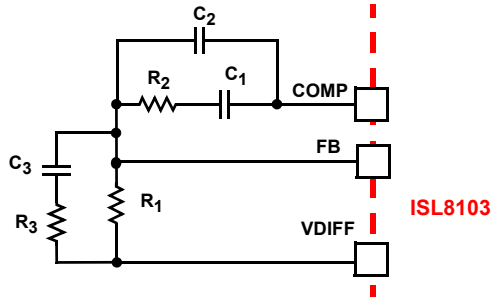
FIGURE 20. COMPENSATION CONFIGURATION FOR NON-LOAD-LINE REGULATED ISL8103 CIRCUIT
