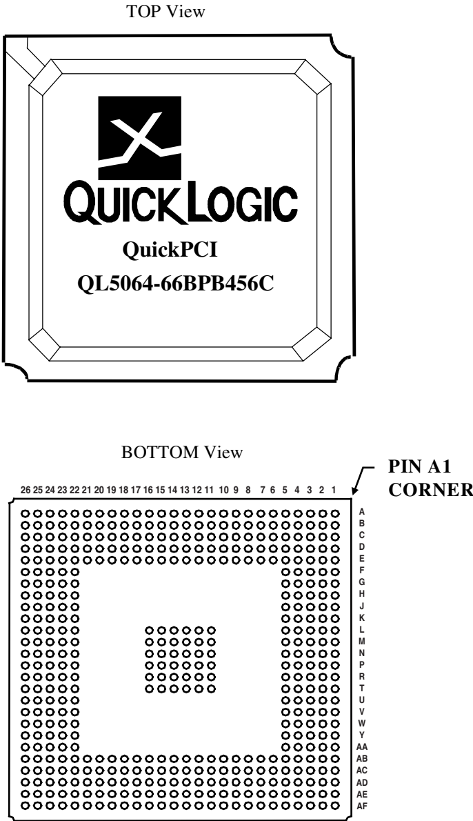
Figure 14: 456 Pin PBGA Pinout Diagram
