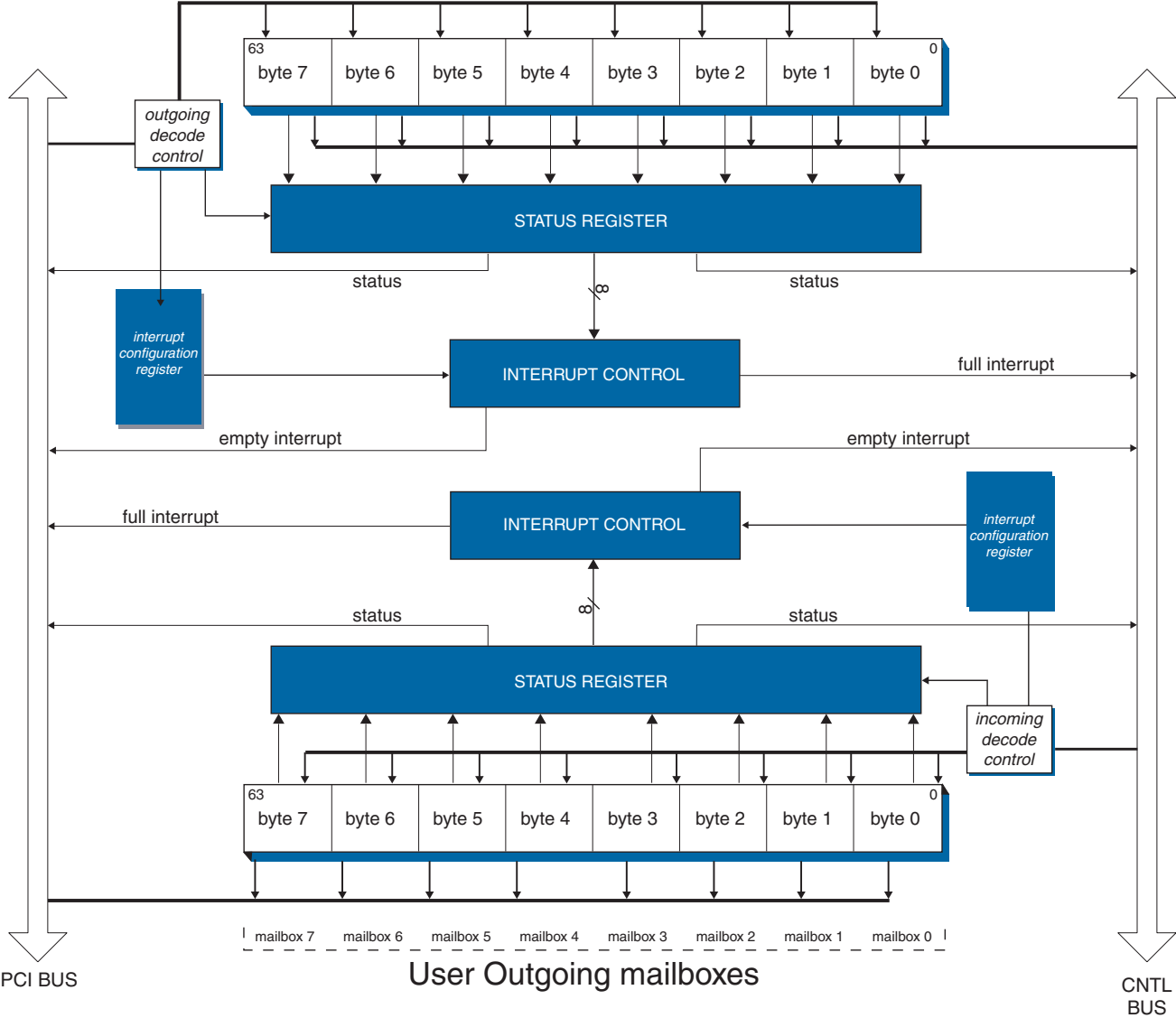
Figure 4: Mailbox Structure
