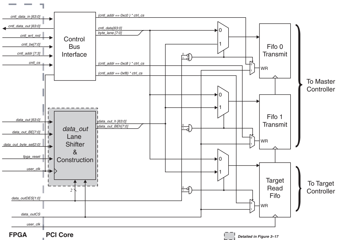
Figure 7: DataOUT and Control Bus Description
