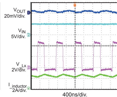
Output Ripple Voltage
