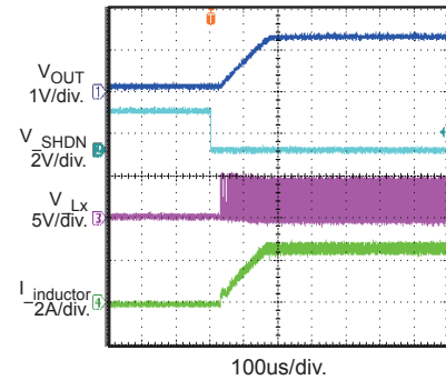
SHDN Start Up with 2.5A Load
