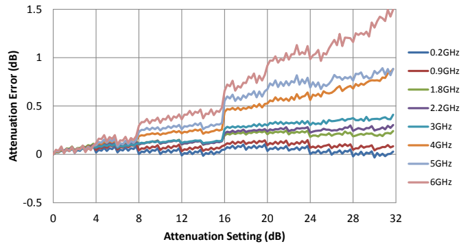
Figure 10. 0.25 dB Attenuation Error vs. Frequency
