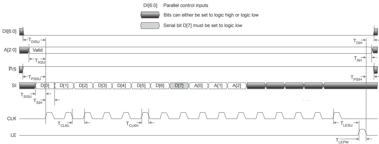
Figure 6. Latched-Parallel/Direct-Parallel Timing Diagram
