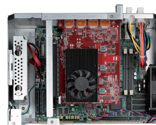
DPX-S1000 internal view with graphic card fitted
