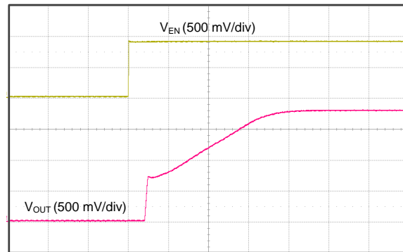
Time (100 \mu\text{s}/\text{div} ) R_L = 6.2\text{ }\Omega , 1- \mu\text{F} output capacitor
