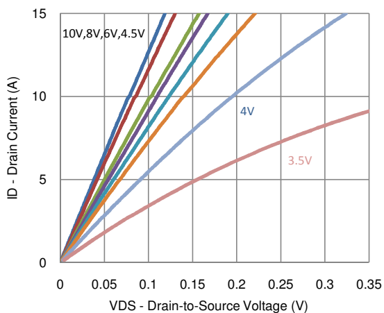
5. Output Characteristics
