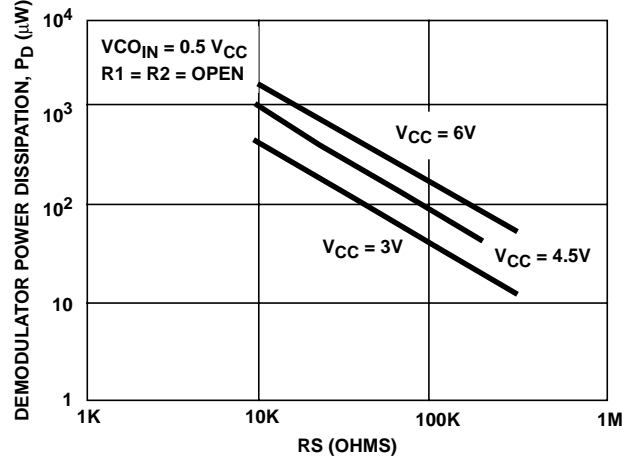
FIGURE 41. HCT7046A DEMODULATOR POWER DISSIPATION vs RS (TYP) ( V_{CC} = 3V, 4.5V, 6V )
