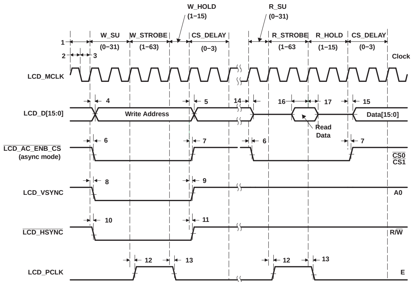
Figure 6-49. Micro-Interface Graphic Display 6800 Read
