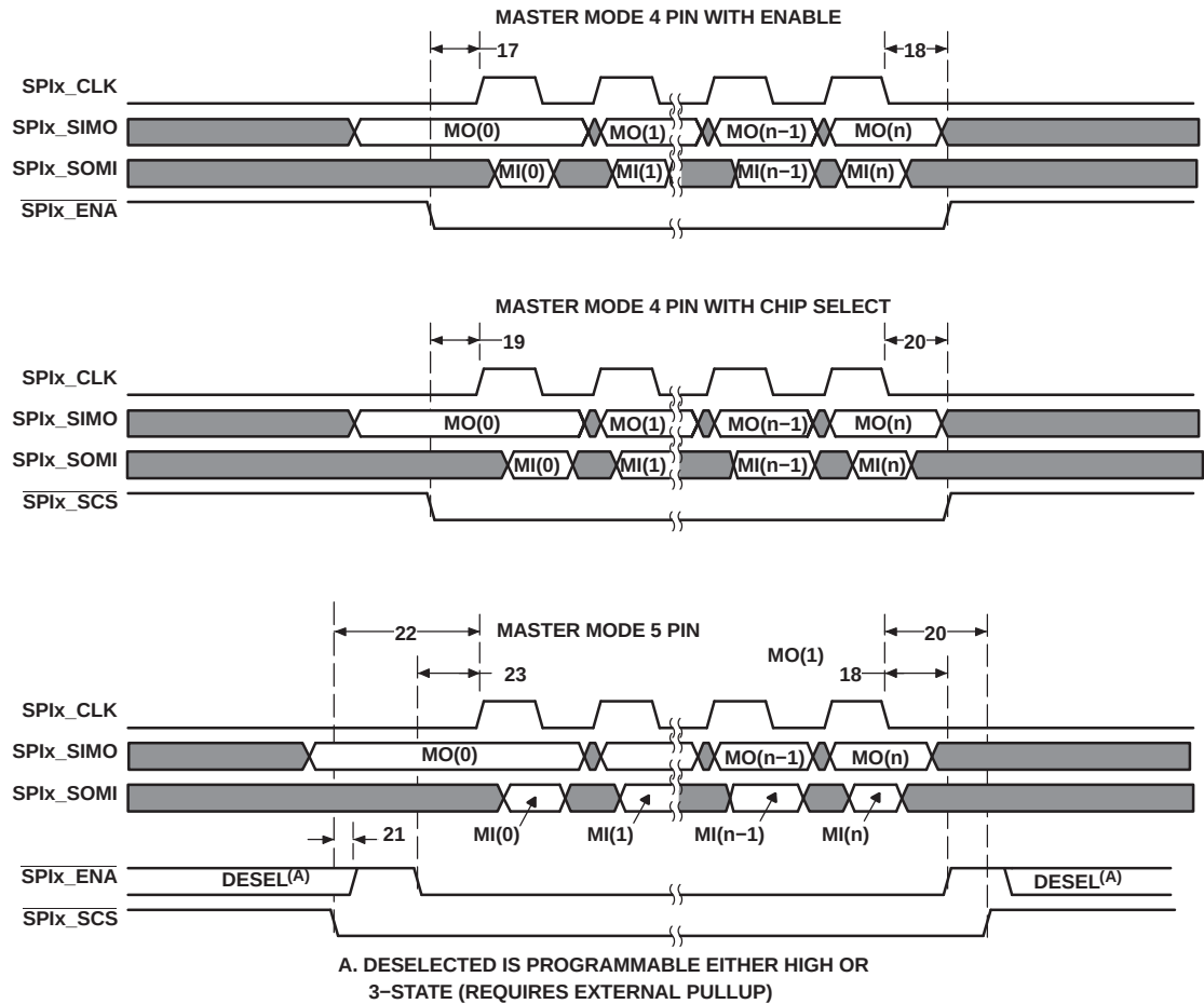
Figure 6-39. SPI Timings—Master Mode (4-Pin and 5-Pin)
