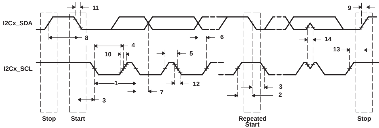
Figure 6-62. I2C Receive Timings
