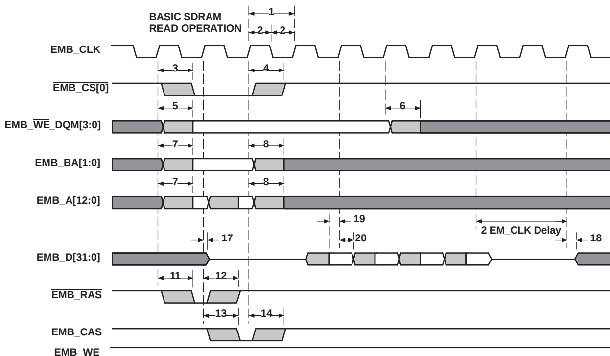
Figure 6-24. EMIFB Basic SDRAM Read Operation
