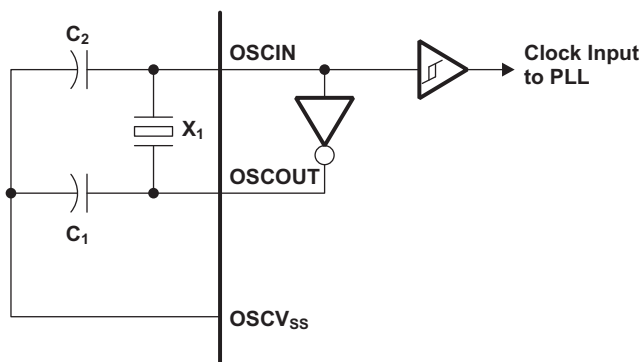
Figure 6-5. On-Chip 1.2V Oscillator
