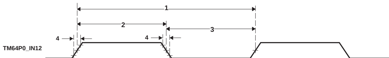
Figure 6-59. Timer Timing
