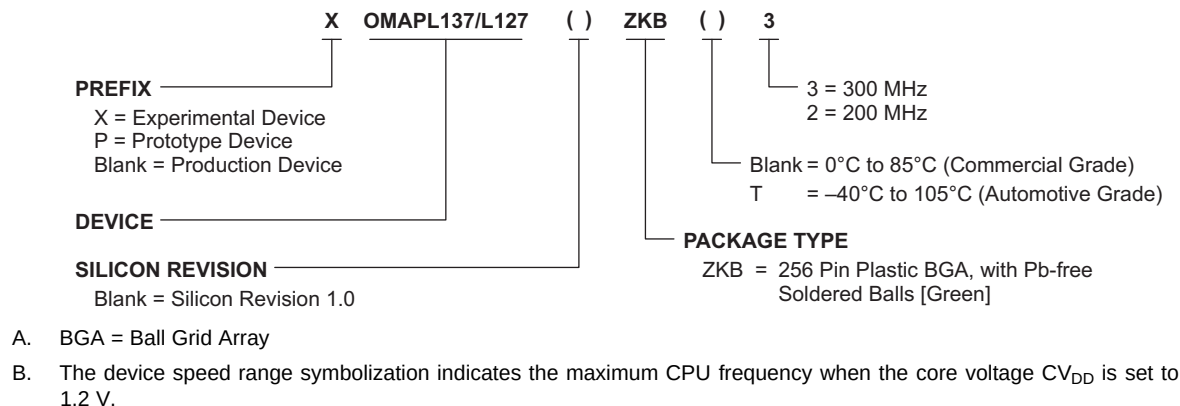
Figure 4-32. Device Nomenclature
