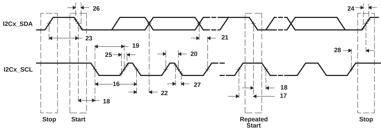
Figure 6-63. I2C Transmit Timings
