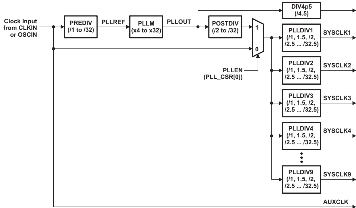
Figure 6-8. PLL Topology
